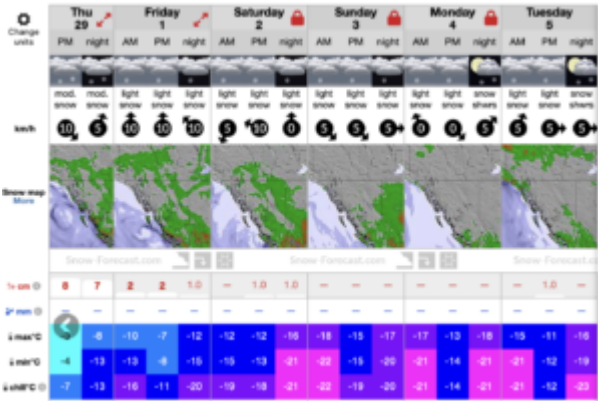
KHMR Snowforecast on Feb 29
